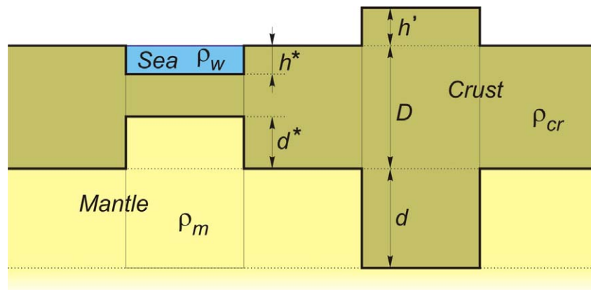
Fig. 1. Airy isostatic model
