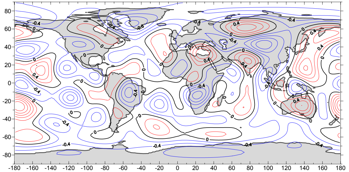
Fig. 3. Optimal crustal parameter function up to spherical harmonic degree K=12
