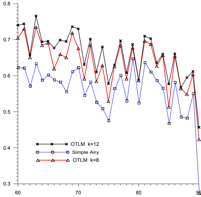
Fig. 5. Geopotential vs. OLTM model correlation spectra for the fit range 60 - 90
