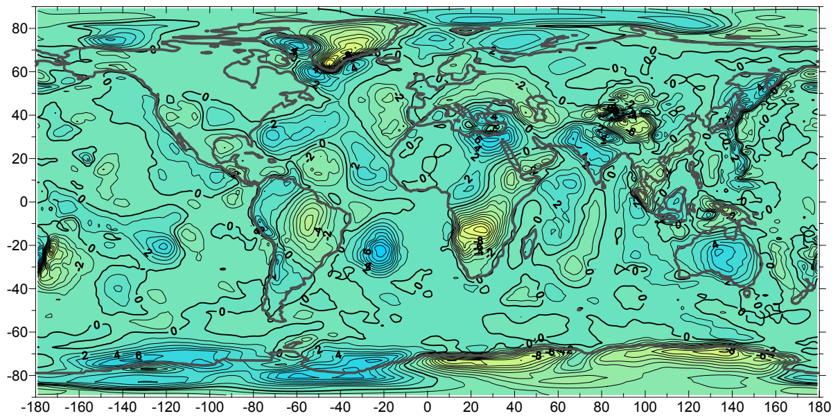
Fig. 4. Optimal topographic-isostatic vs. Airy model geoid height differences for K=12 model
