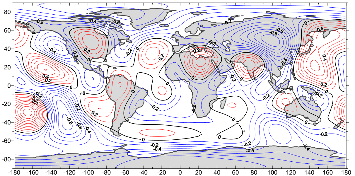
Fig. 2. Optimal crustal parameter function up to spherical harmonic degree K=8
